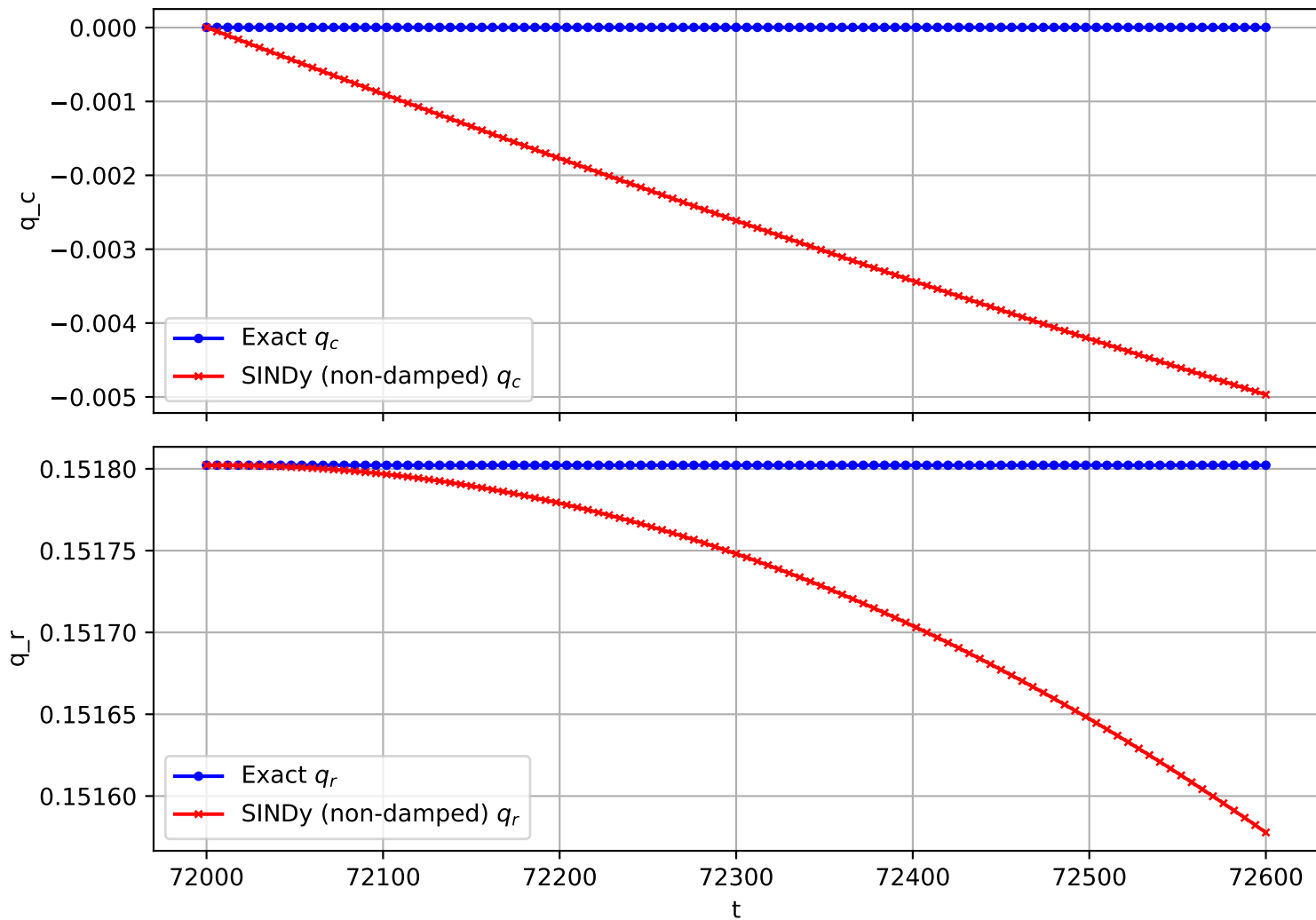
Trajectory 1035 (non-damped)
