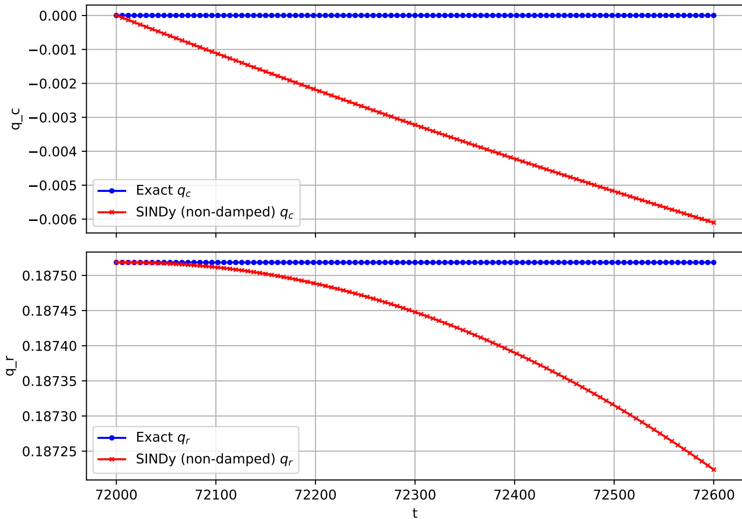
Trajectory 1037 (non-damped)
