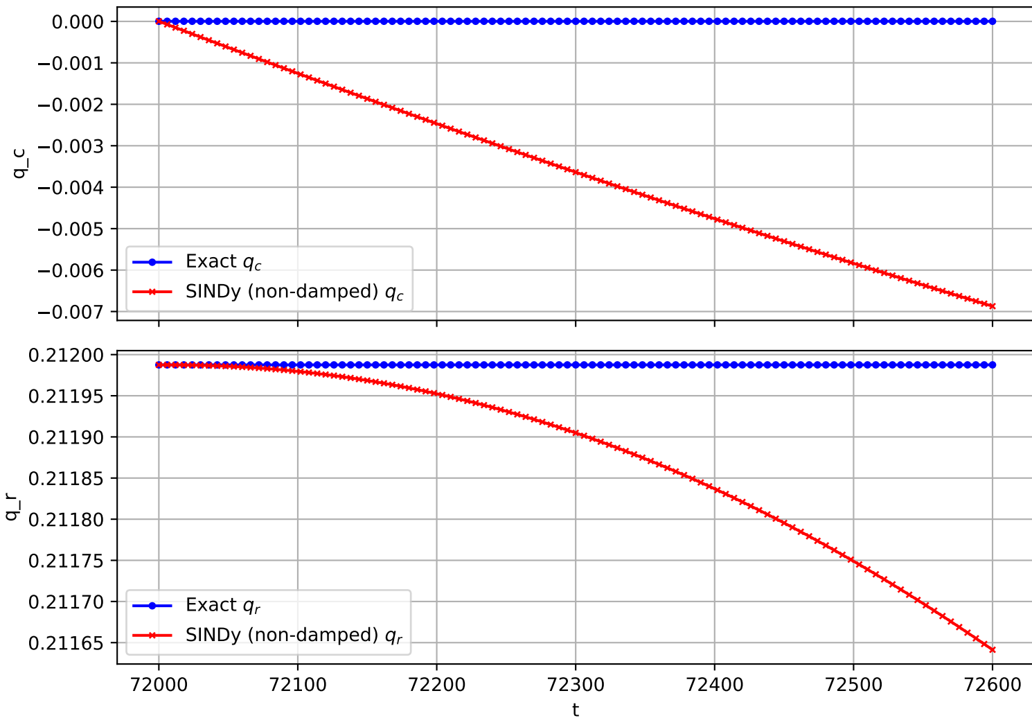
Trajectory 1040 (non-damped)
