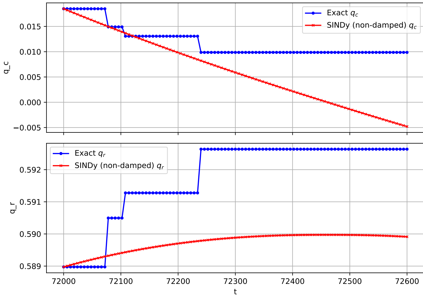
Trajectory 1049 (non-damped)
