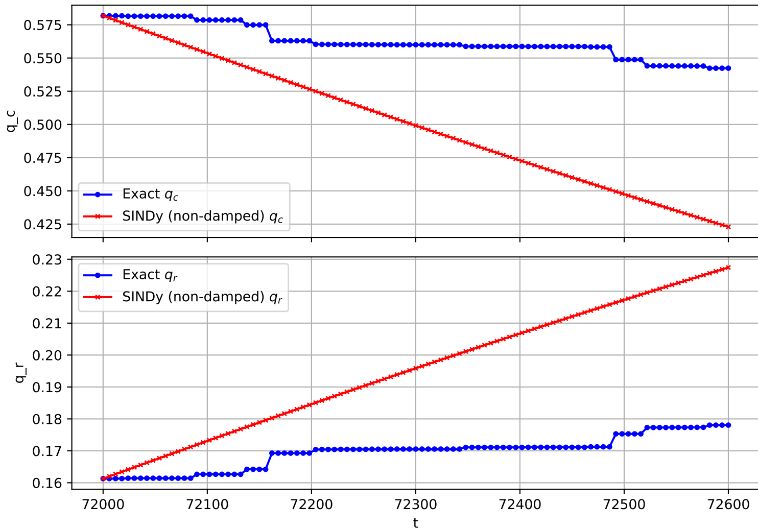
Trajectory 1058 (non-damped)
