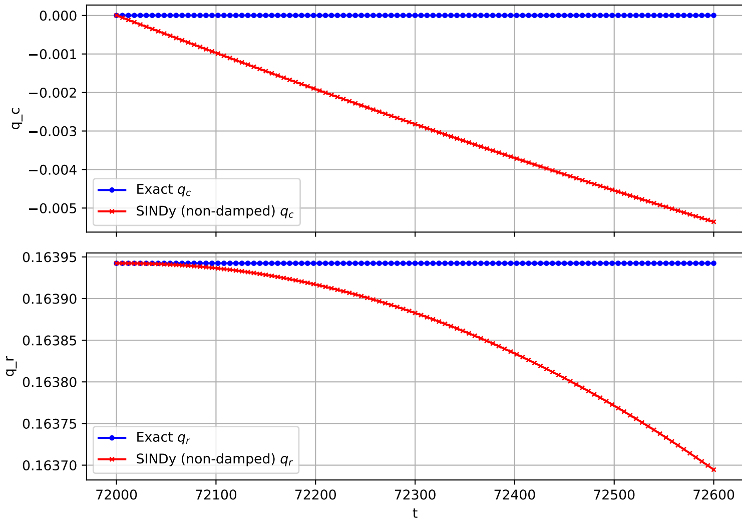
Trajectory 1061 (non-damped)
