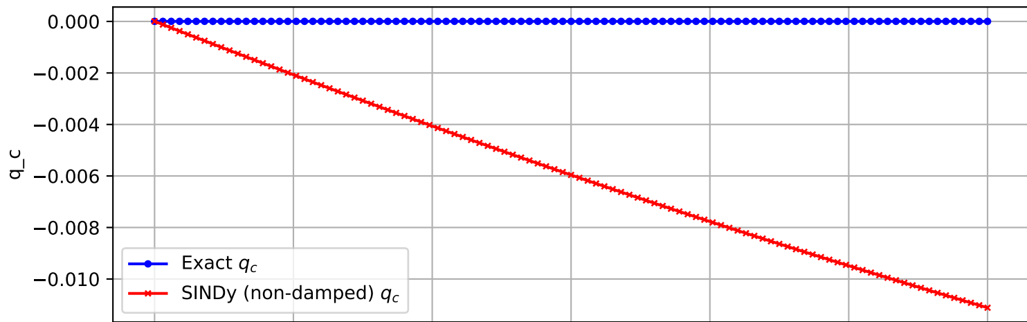
Trajectory 1064 (non-damped)
