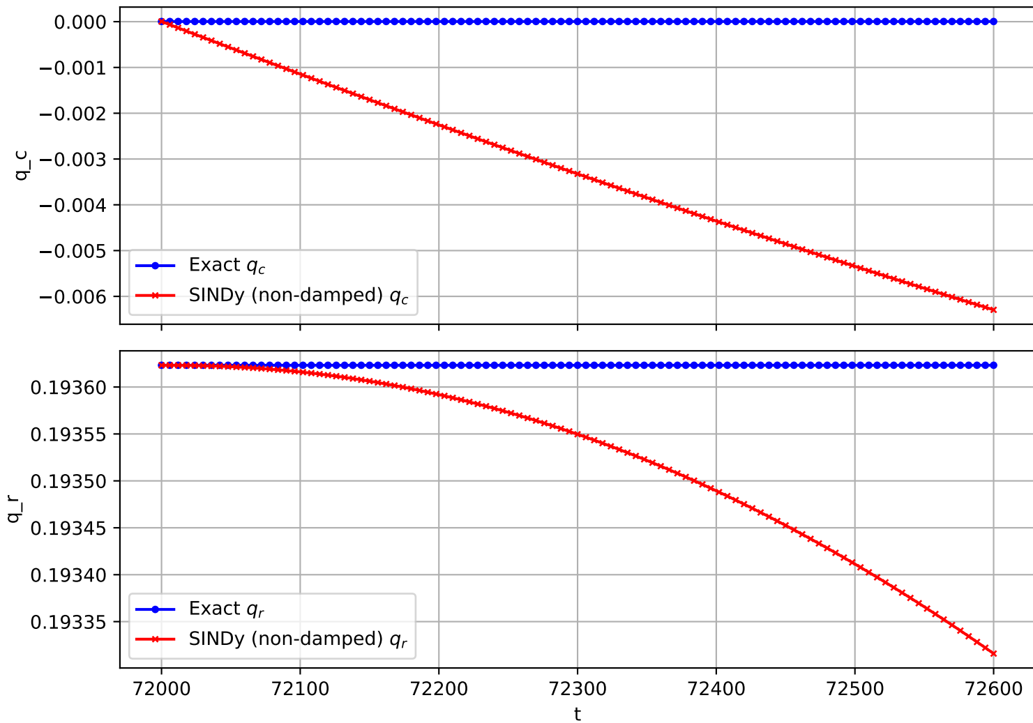
Trajectory 1069 (non-damped)
