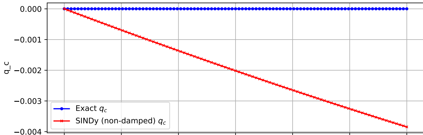
Trajectory 1073 (non-damped)
