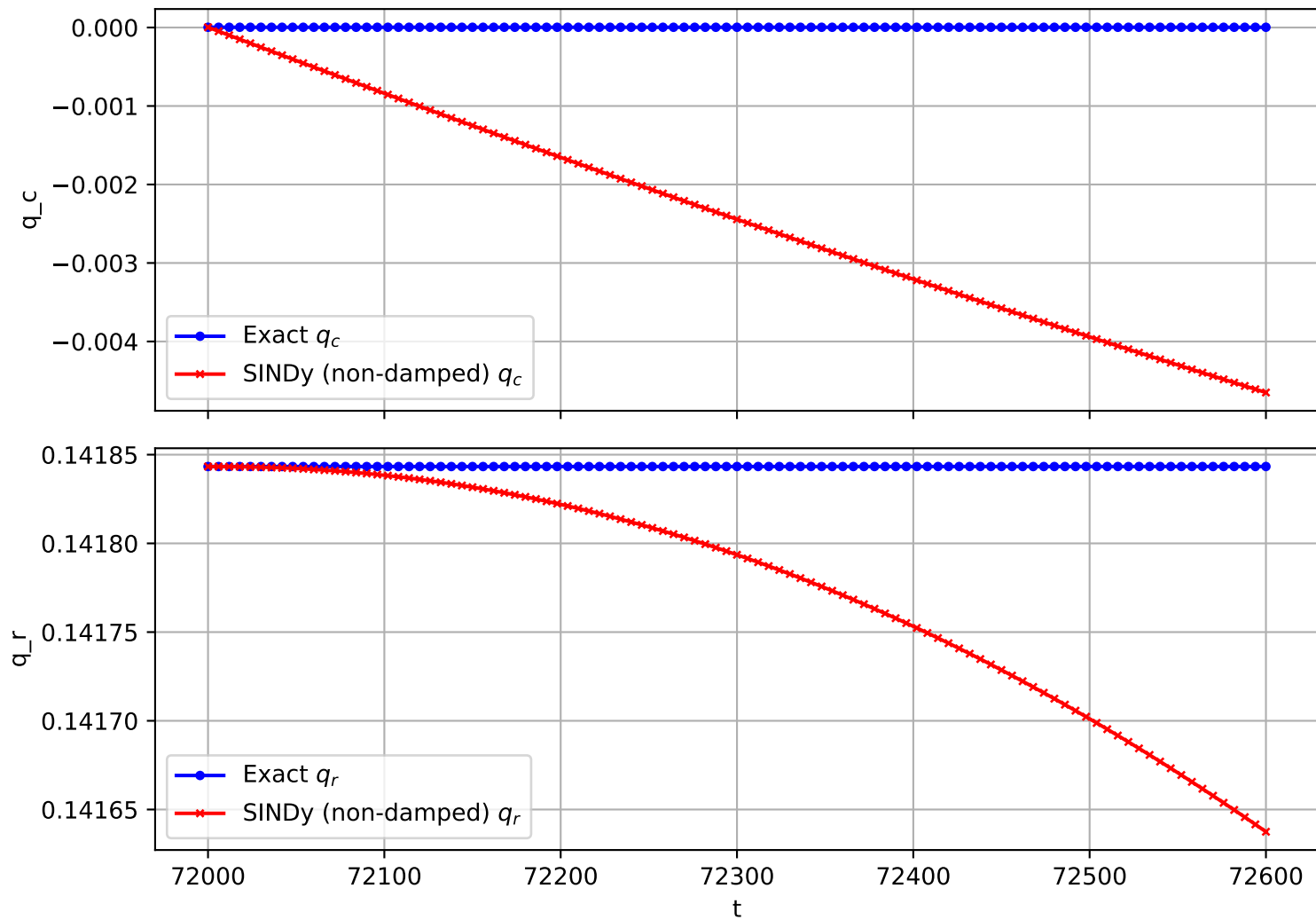
Trajectory 1077 (non-damped)
