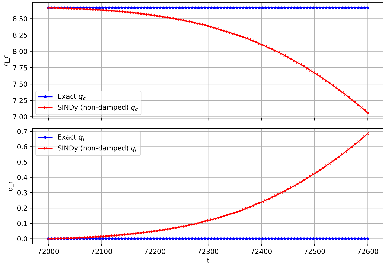
Trajectory 1082 (non-damped)
