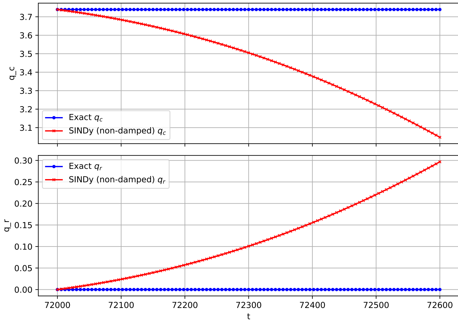
Trajectory 1085 (non-damped)
