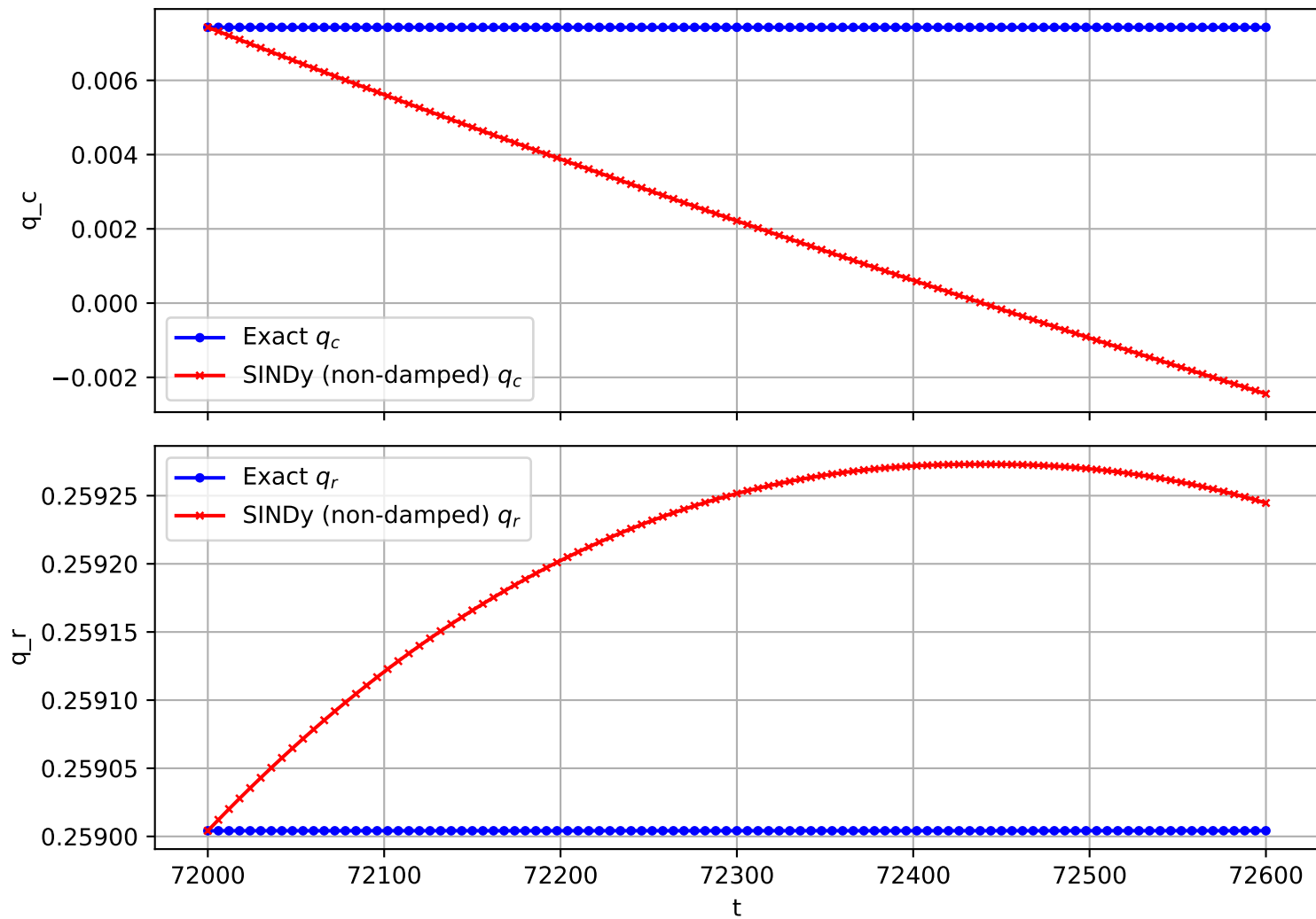
Trajectory 1092 (non-damped)
