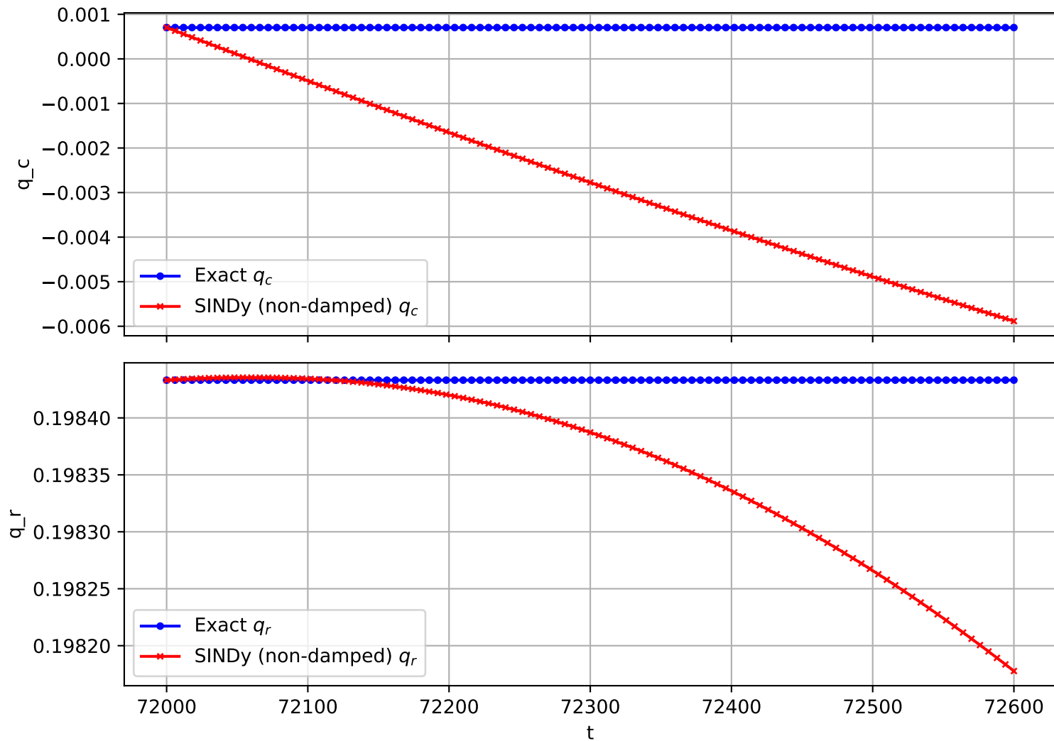
Trajectory 1104 (non-damped)
