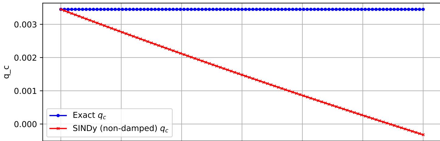
Trajectory 1106 (non-damped)
