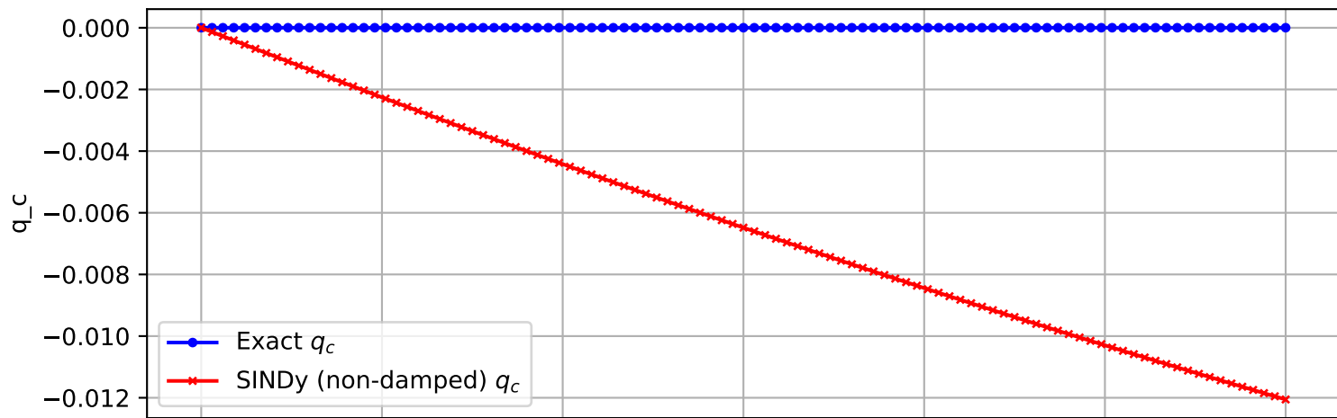
Trajectory 1108 (non-damped)
