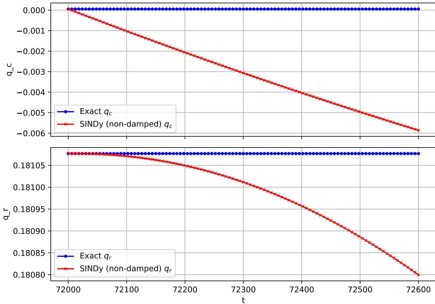
Trajectory 1110 (non-damped)
