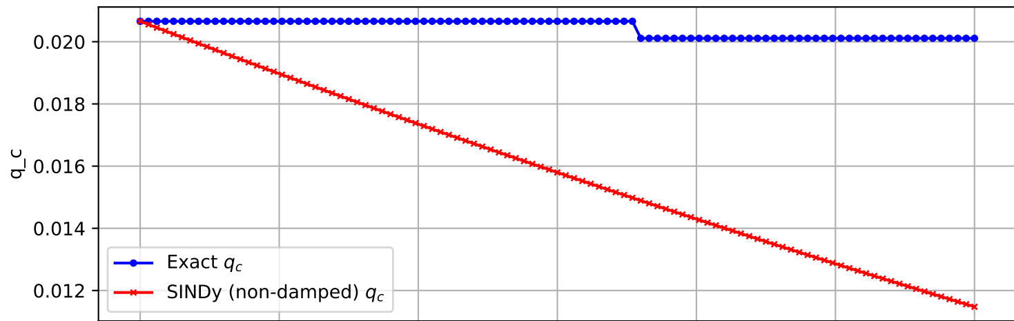
Trajectory 1113 (non-damped)
