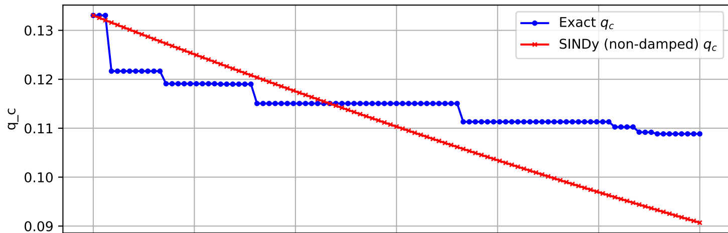
Trajectory 1117 (non-damped)
