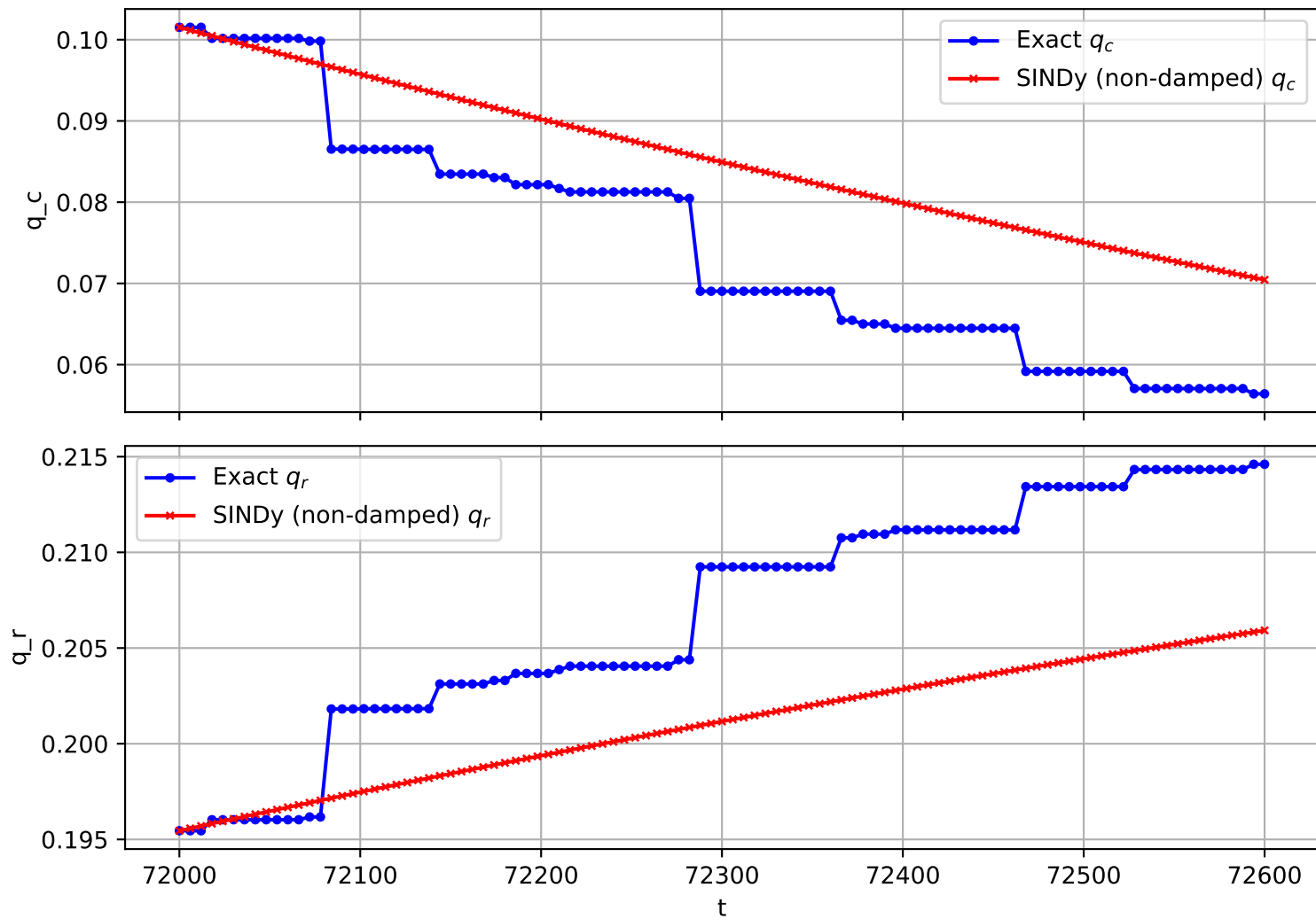
Trajectory 1129 (non-damped)
