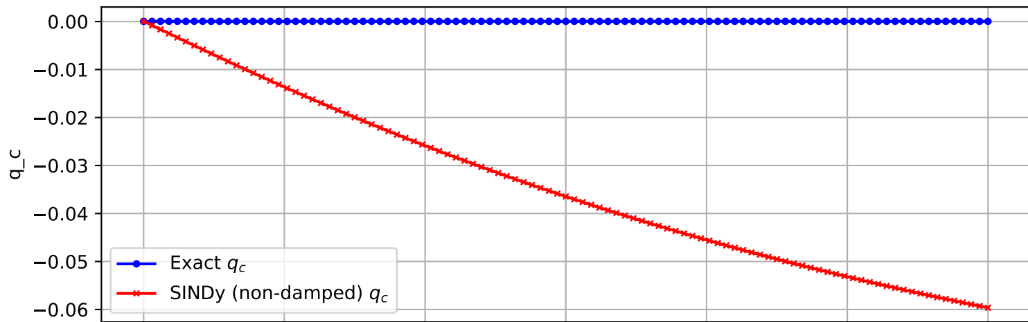
Trajectory 1132 (non-damped)
