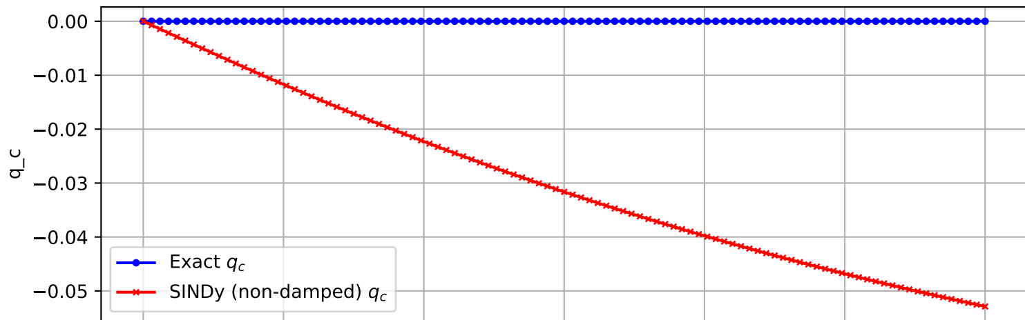
Trajectory 1135 (non-damped)
