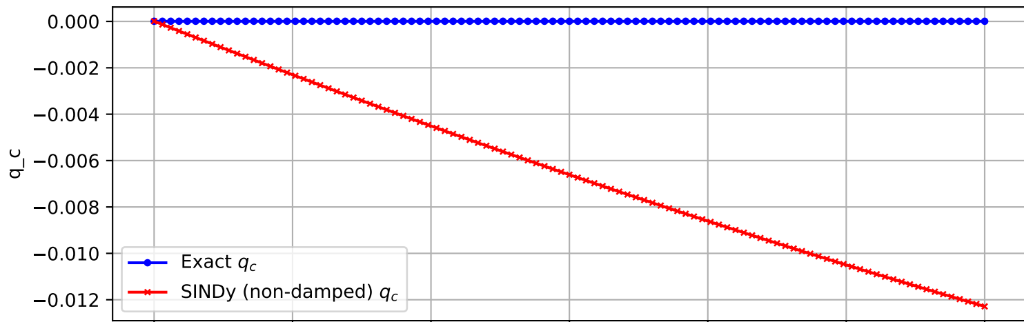
Trajectory 116 (non-damped)
