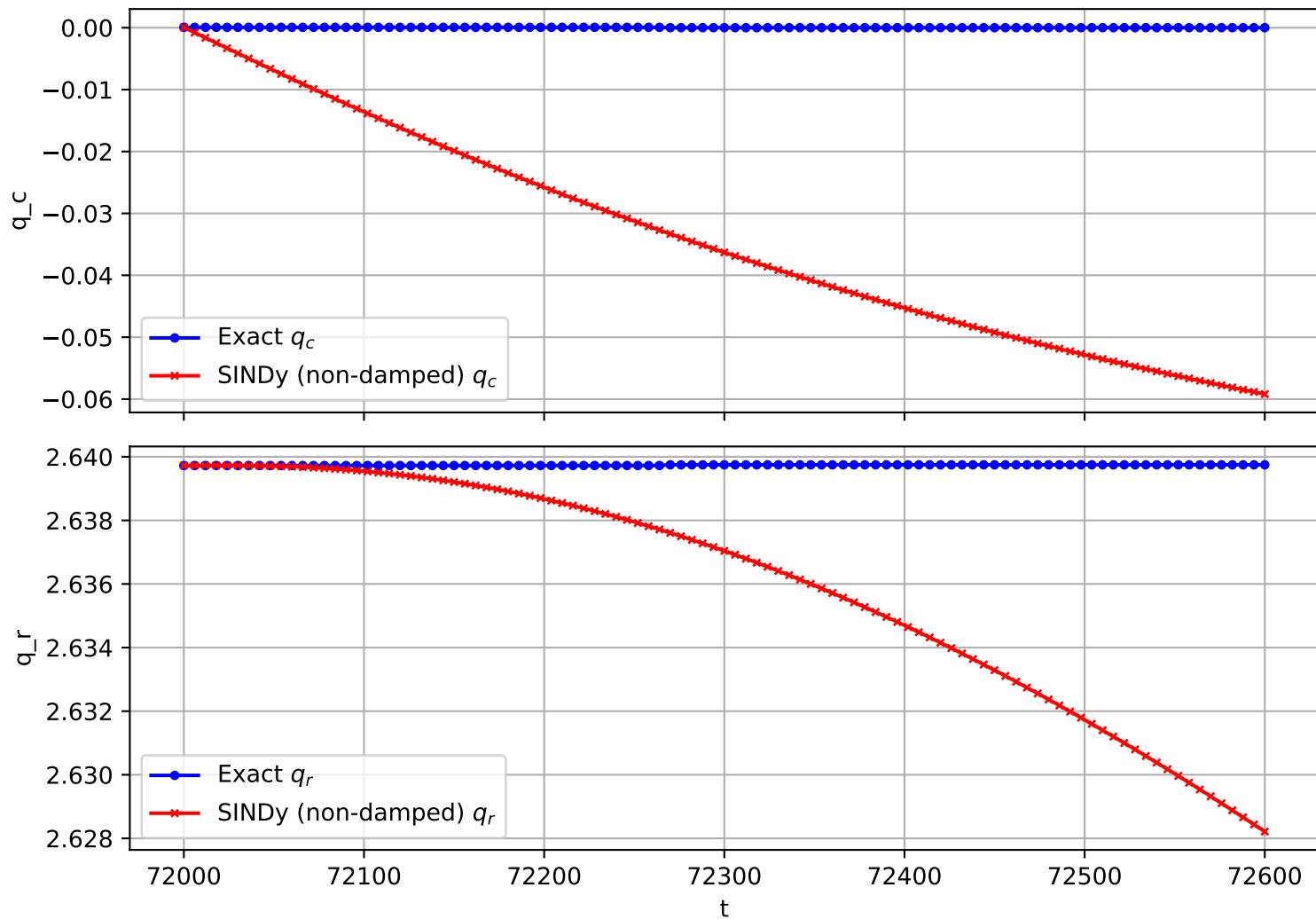
Trajectory 1160 (non-damped)
