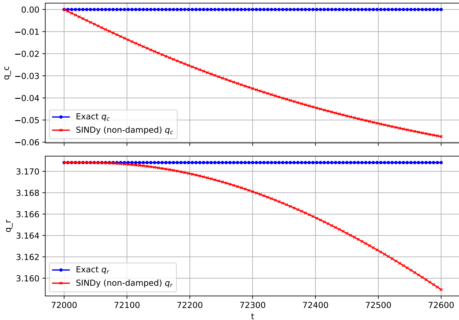
Trajectory 1169 (non-damped)
