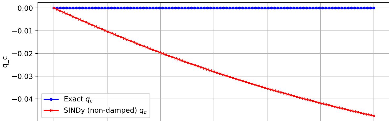
Trajectory 1174 (non-damped)
