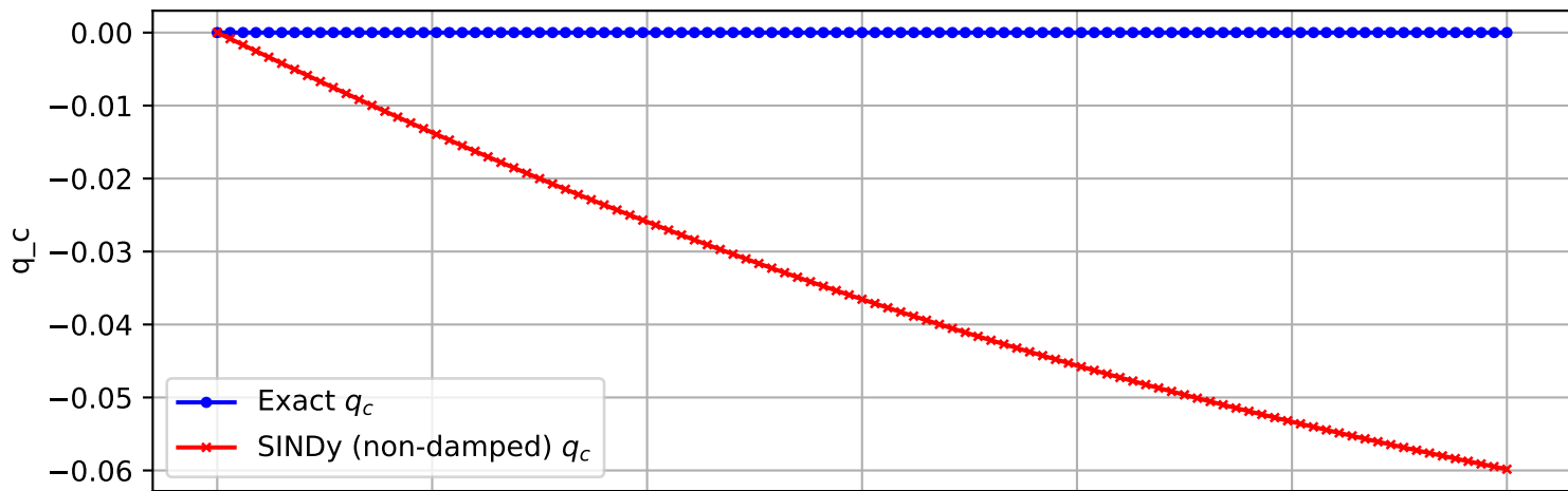
Trajectory 1178 (non-damped)
