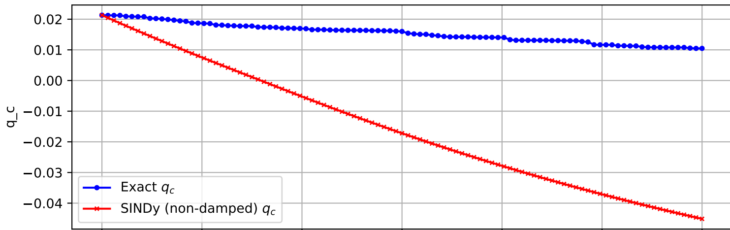
Trajectory 1179 (non-damped)
