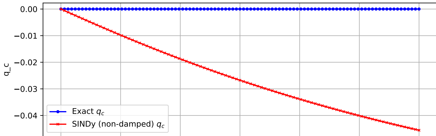
Trajectory 118 (non-damped)
