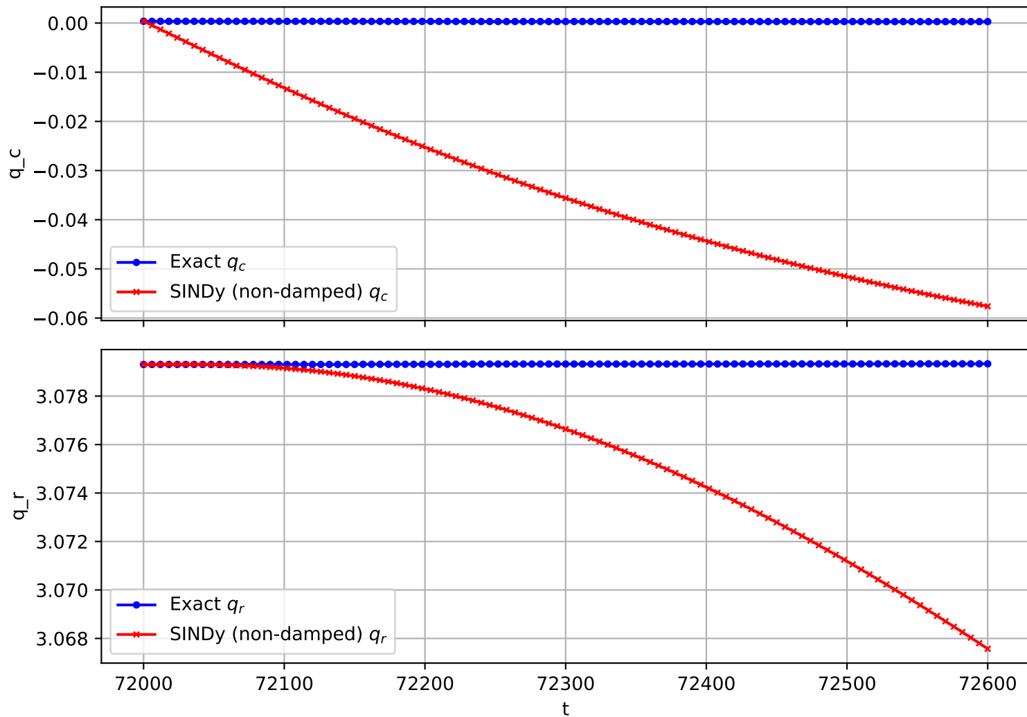
Trajectory 120 (non-damped)
