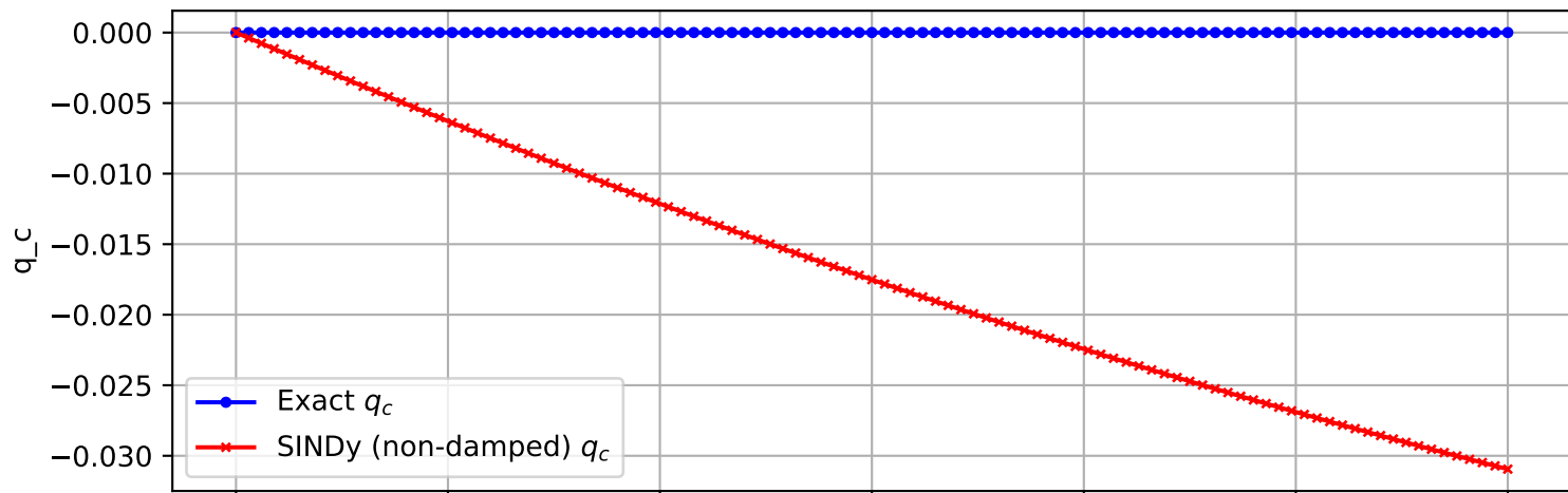
Trajectory 1209 (non-damped)
