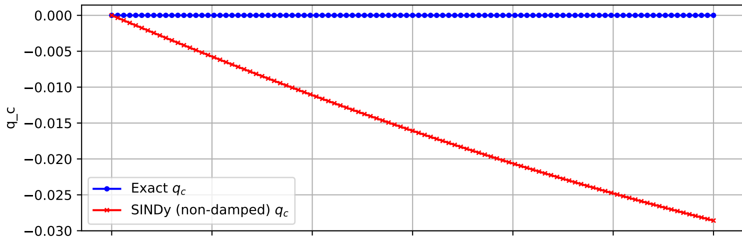
Trajectory 1213 (non-damped)
