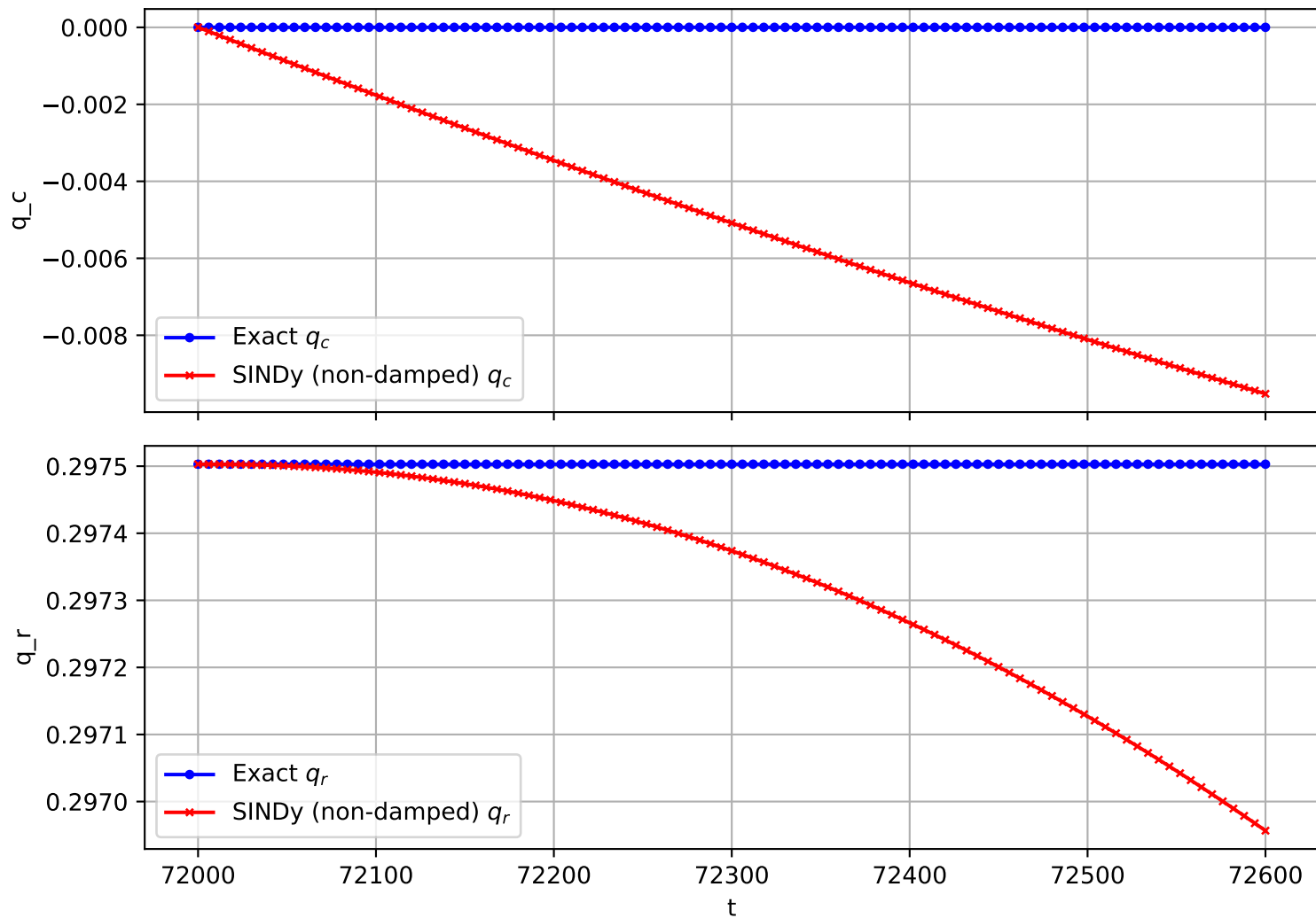
Trajectory 1233 (non-damped)
