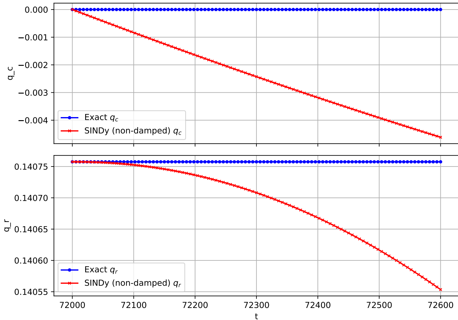
Trajectory 1235 (non-damped)
