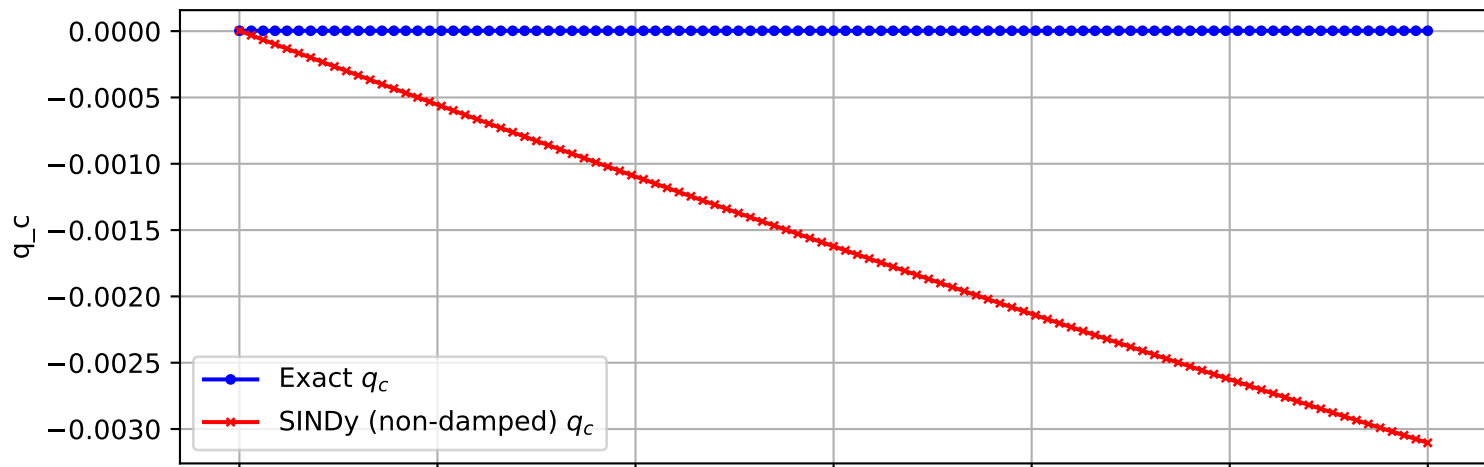
Trajectory 1261 (non-damped)
