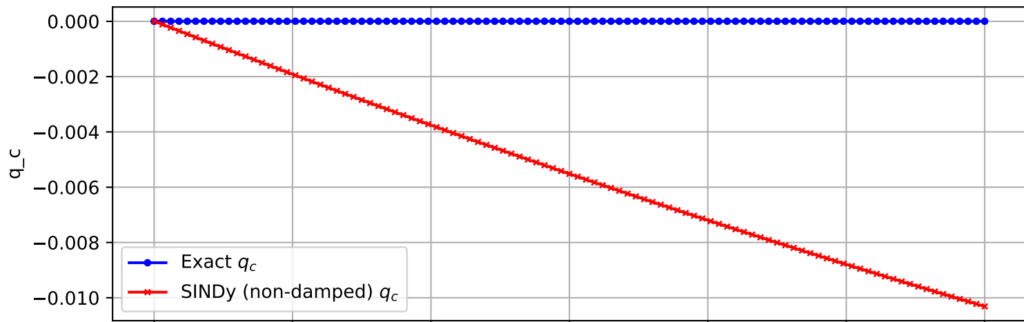
Trajectory 1269 (non-damped)
