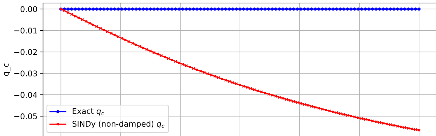
Trajectory 1277 (non-damped)
