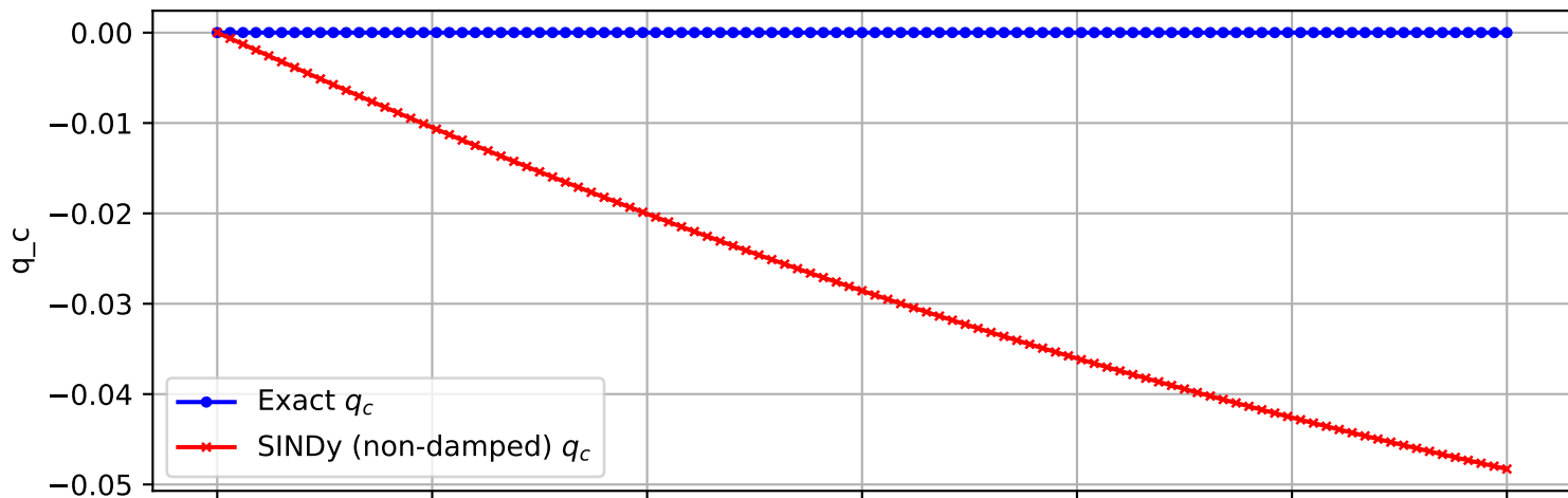
Trajectory 1285 (non-damped)
