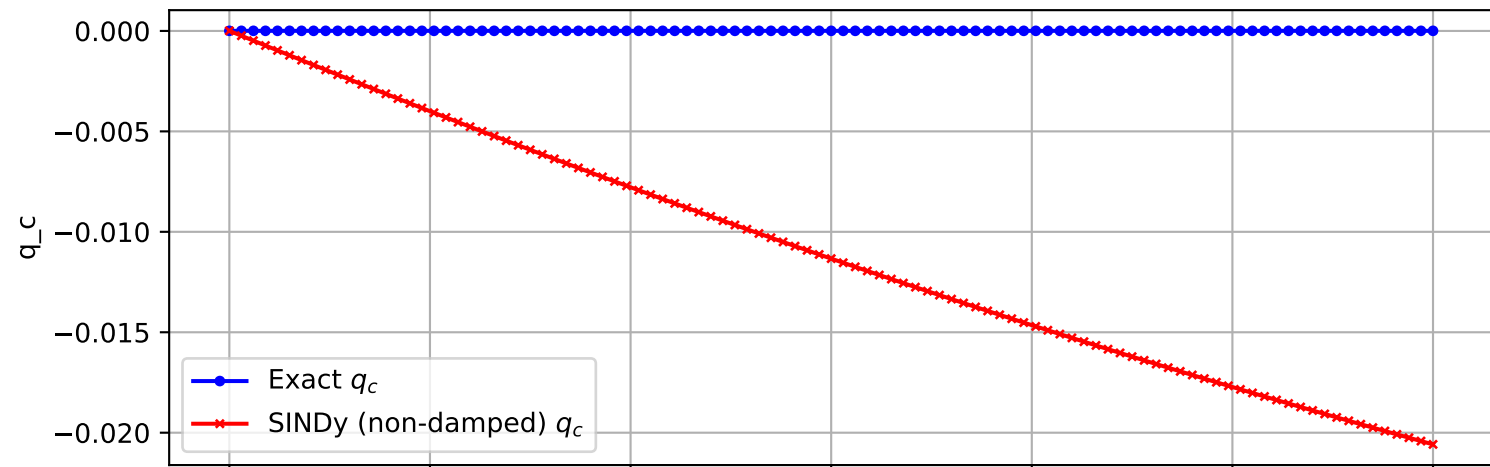
Trajectory 1289 (non-damped)
