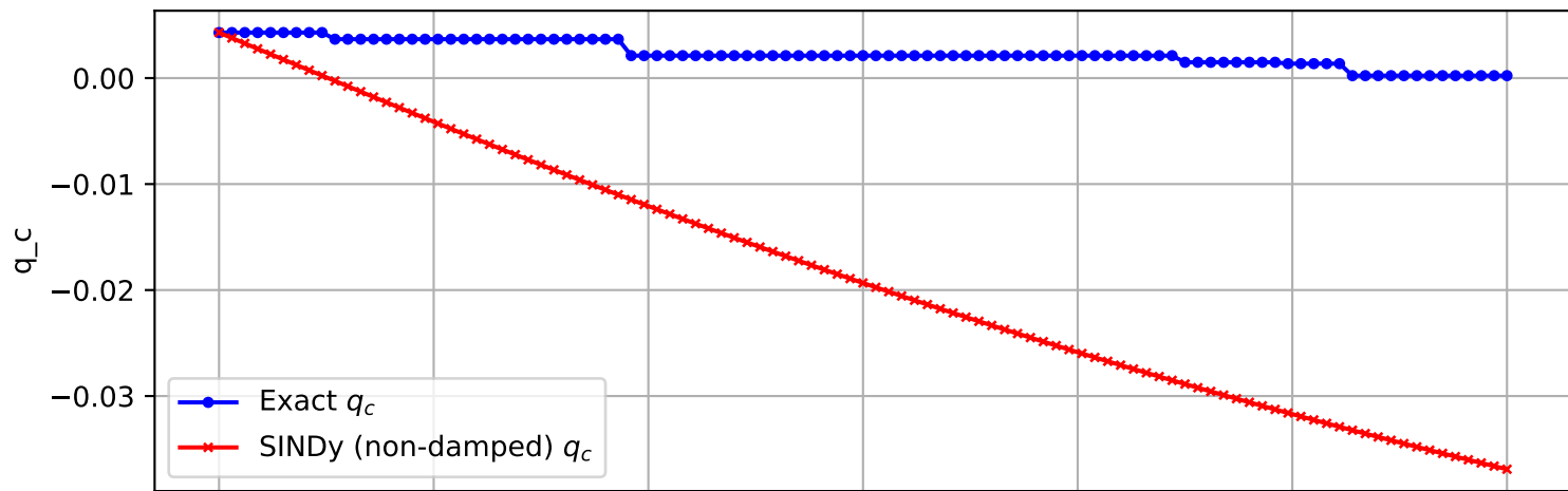
Trajectory 1293 (non-damped)
