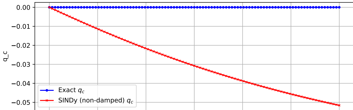
Trajectory 1297 (non-damped)
