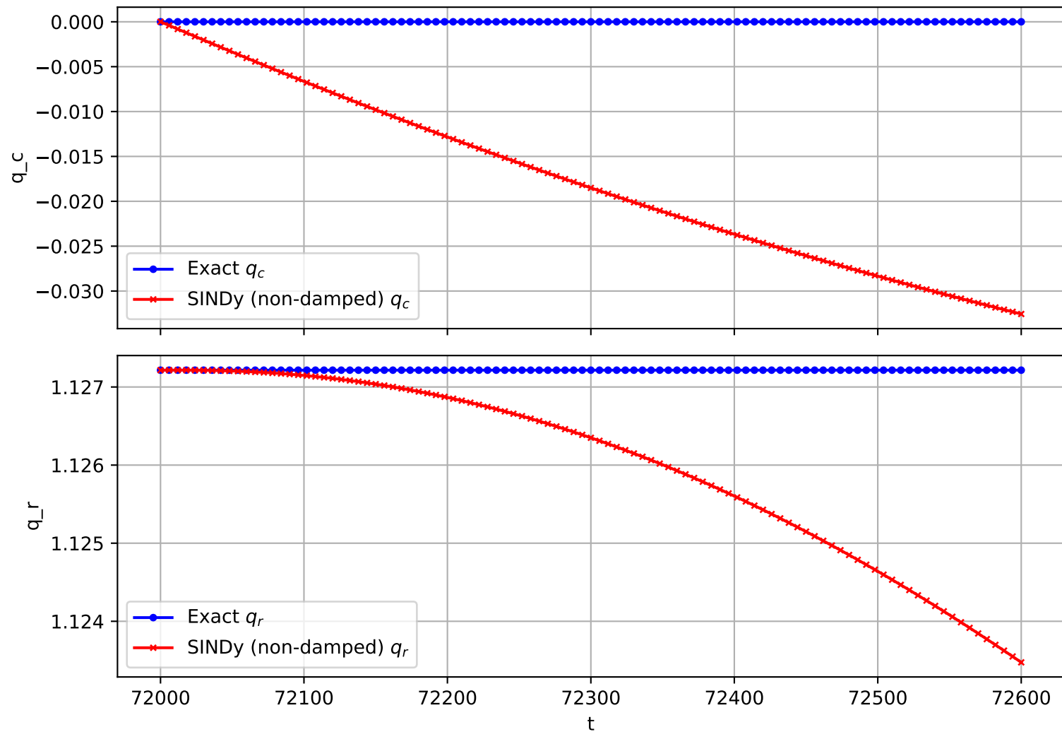
Trajectory 1298 (non-damped)
