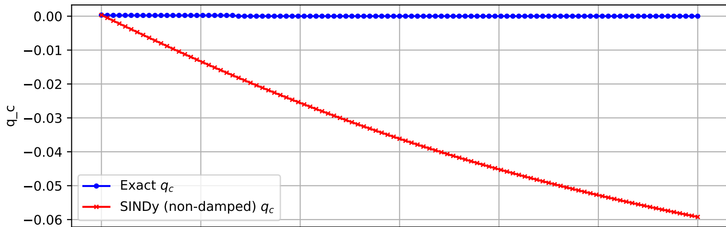
Trajectory 1312 (non-damped)
