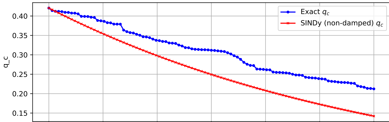
Trajectory 1314 (non-damped)
