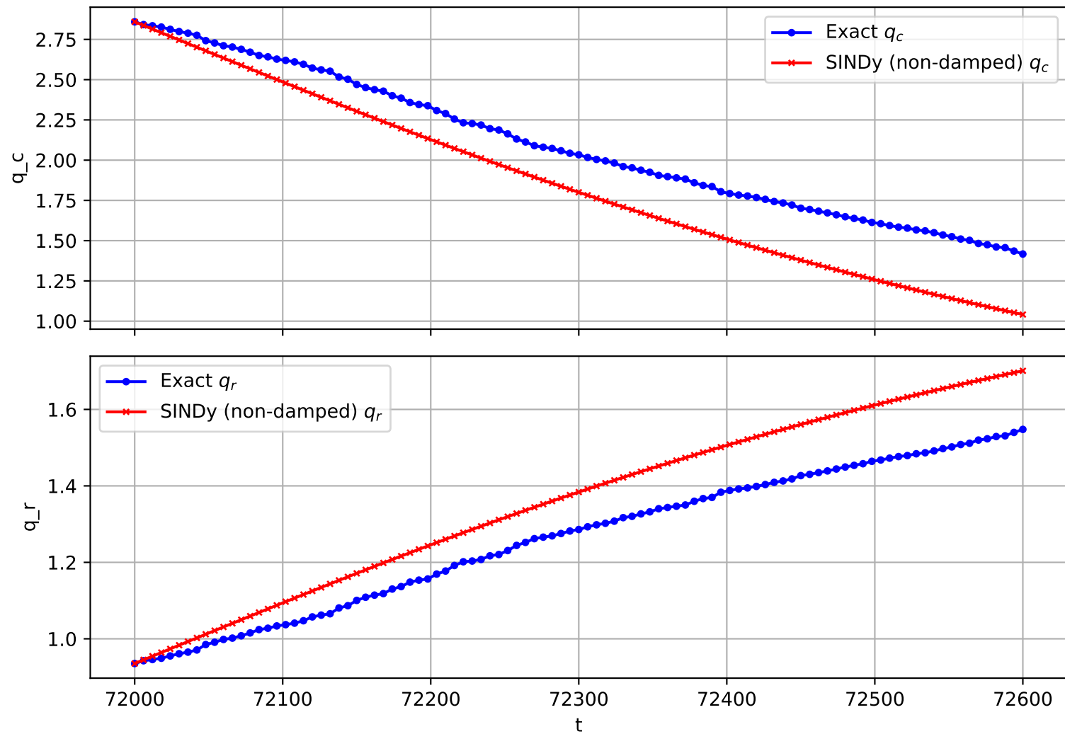
Trajectory 1315 (non-damped)
