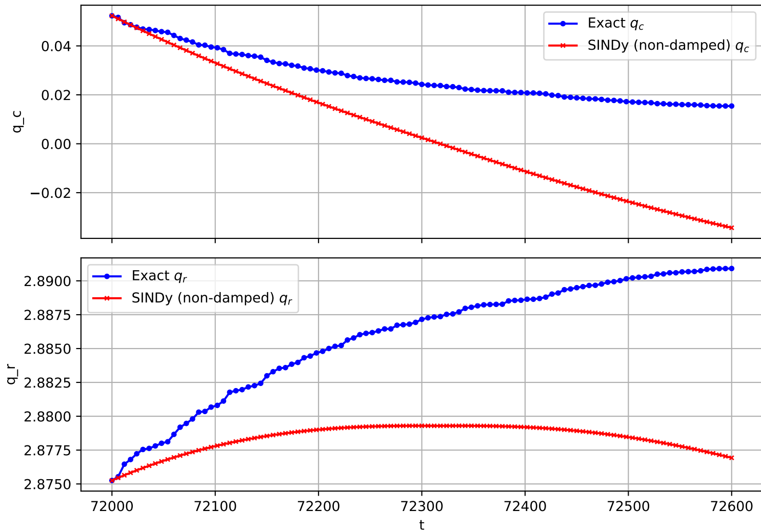
Trajectory 1328 (non-damped)
