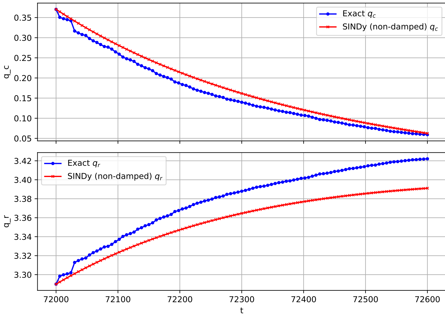
Trajectory 1330 (non-damped)
