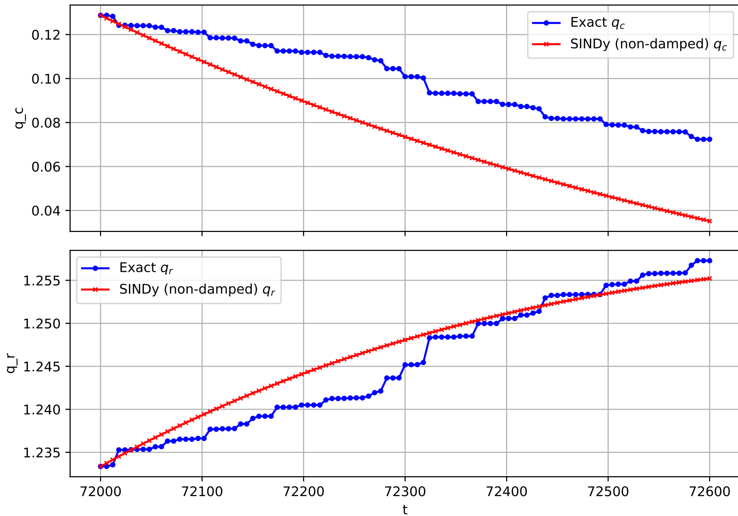
Trajectory 1336 (non-damped)
