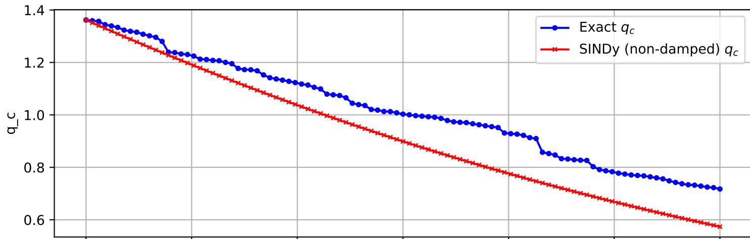
Trajectory 1337 (non-damped)
