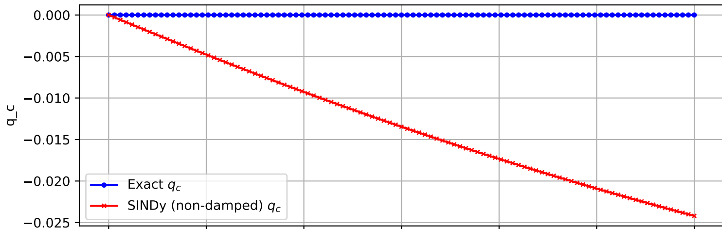
Trajectory 1340 (non-damped)
